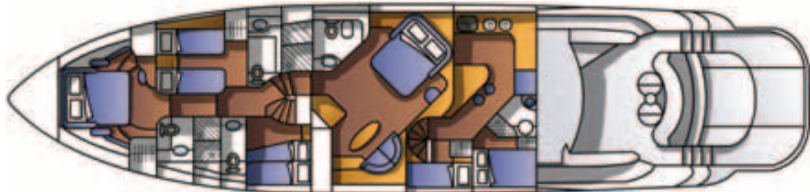
ACCOMMODATION LAYOUT
